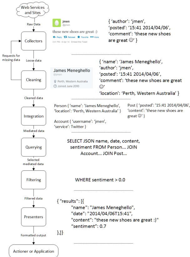
Figure 4: Example data flow within framework
